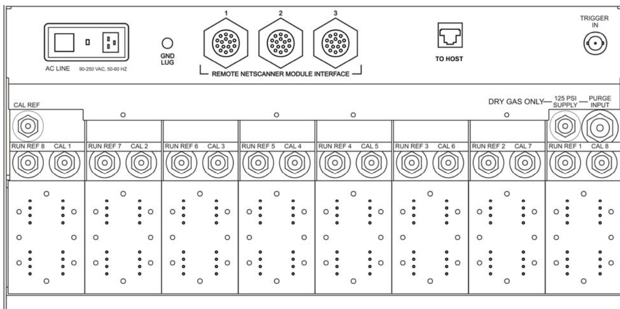
98RK-1 Scanner Interface Rack Rear Panel Layout
