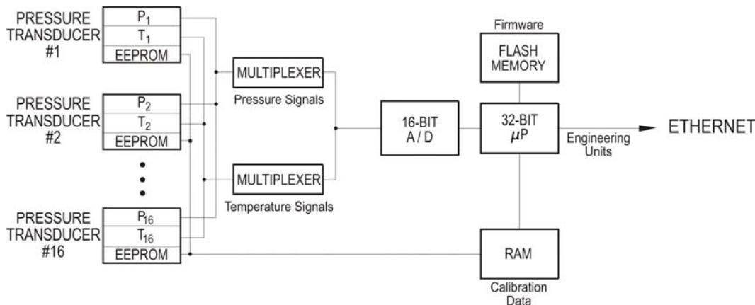
Digital Sensor Temperature Compensation Functional Diagram
