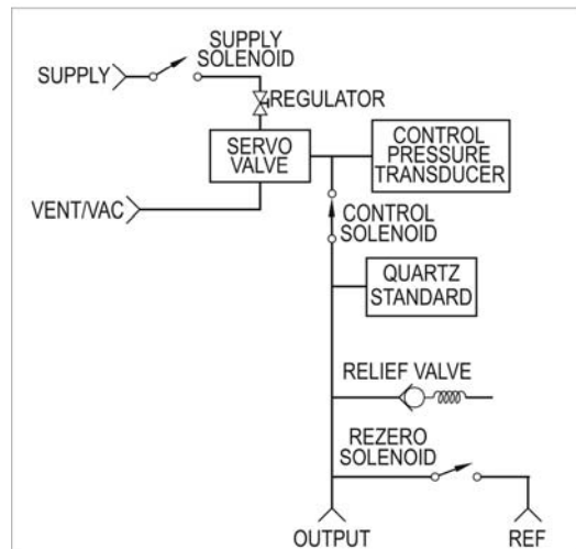
9038 PRESSURE CONTROLLER
